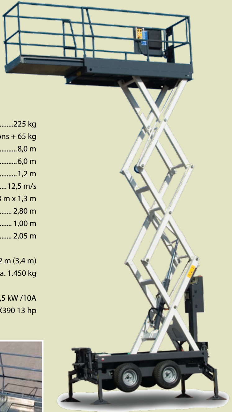
Platform extension 1,2 m (option)
